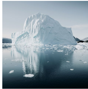
ICEBERG
